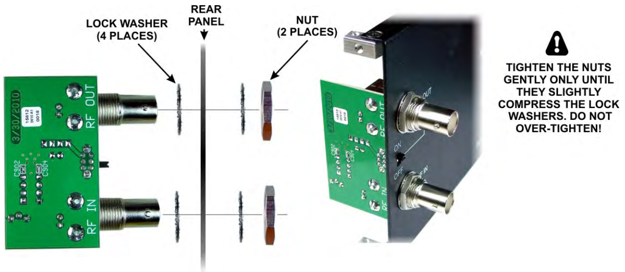
Figure 17. RF Board Installation.
