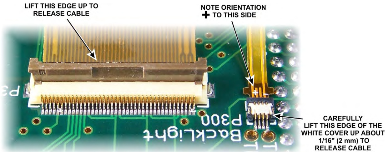
Figure 24. LCD Cable Connectors Opened.
